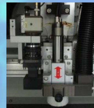
Upper Suction
